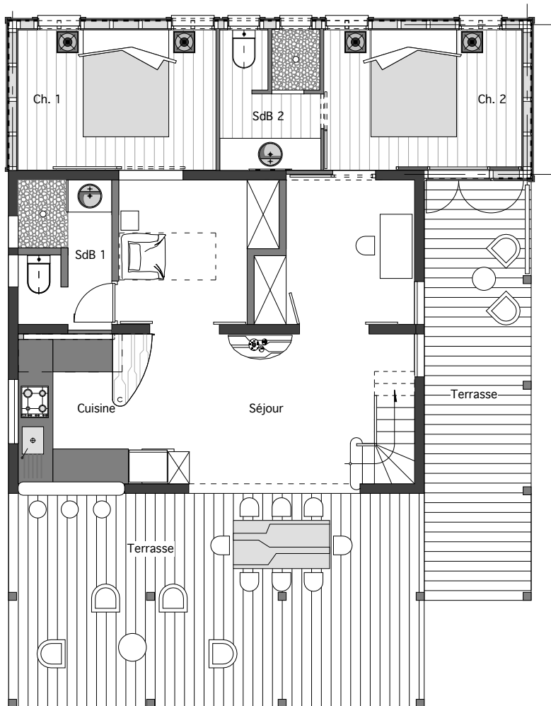
Plan RDC ech: 1/100°
